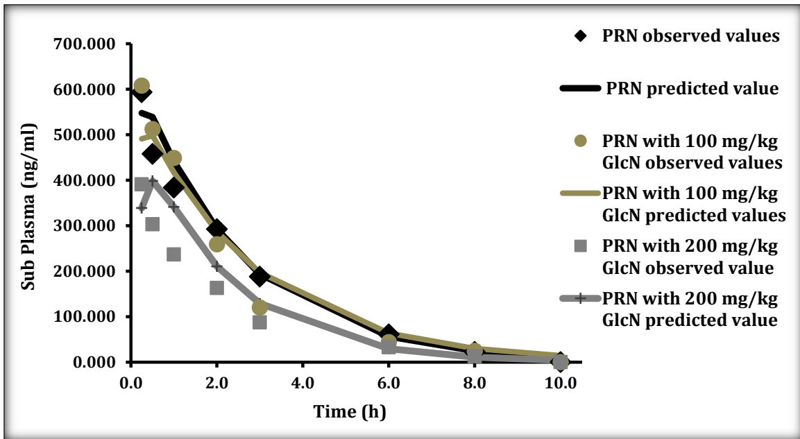
Figure 3.21 Observed versus SimCYP-predicted propranolol plasma concentrations of 20 mg/kg propranolol, propranolol with 100 mg/kg glucosamine and propranolol with 200 mg/kg glucosamine.
